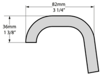
Rim Detail
