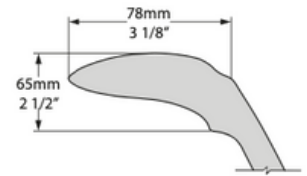
Rim Detail
