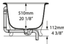
Section BB
