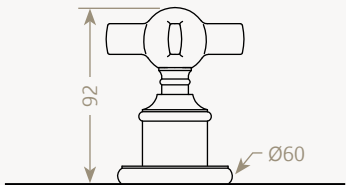
Bain-douche / Bath-shower
